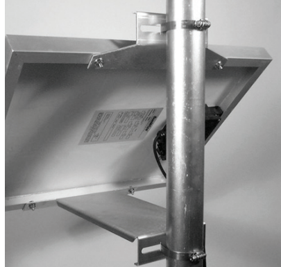
Photo at far left: Adjustable Mount Tilt angle from 15° to 90°
